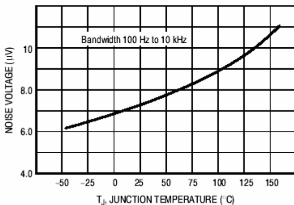
Figure 16. Output Noise
