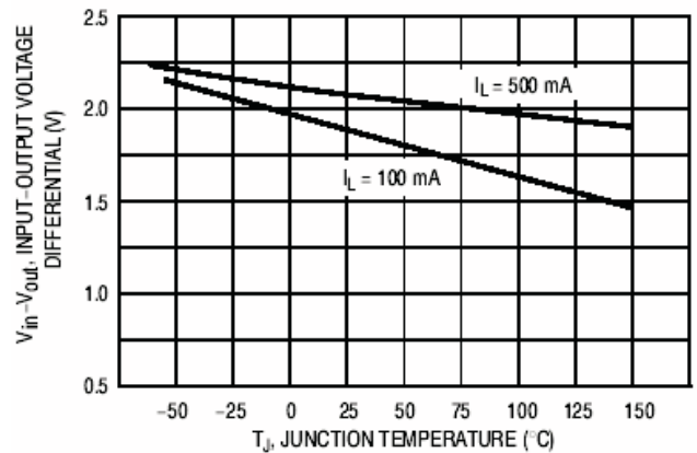
Figure 10. Dropout Voltage
